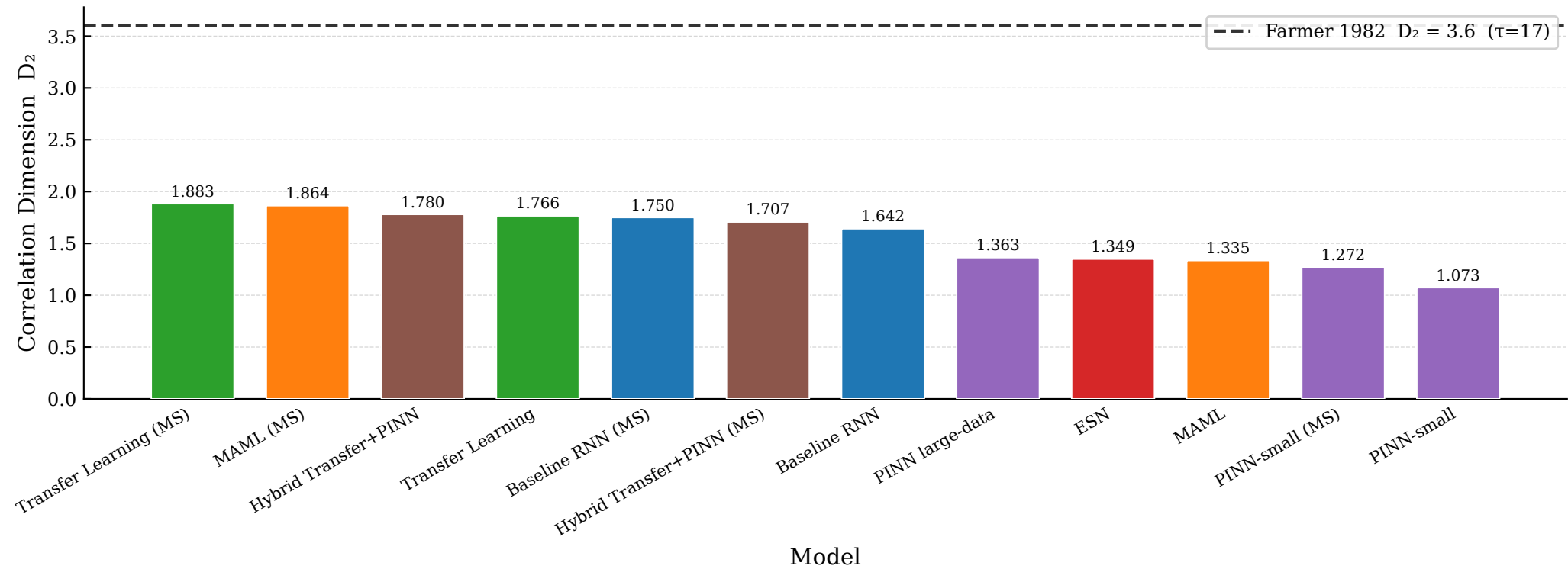
MG — Correlation Dimension D_2 Closer to reference line = better attractor reconstruction
